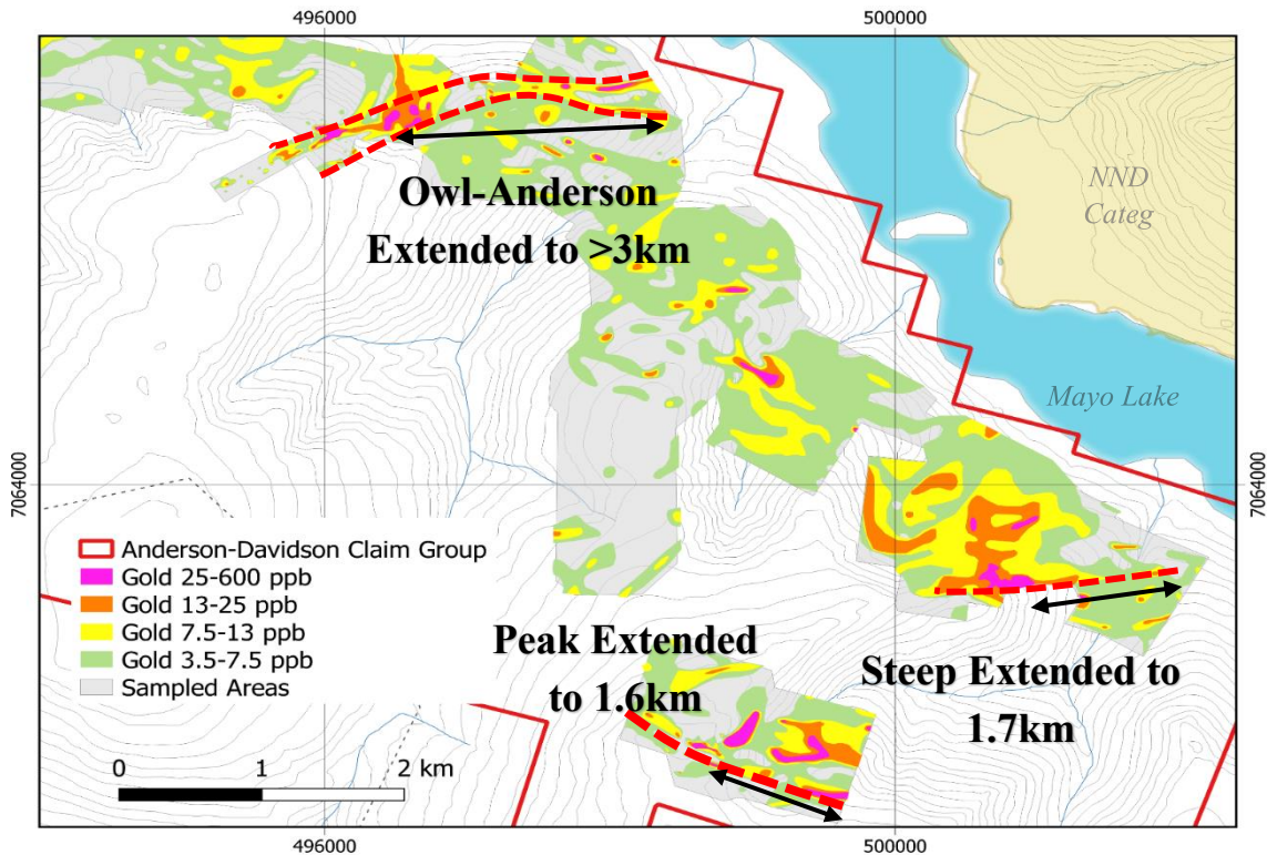
Eastern Anderson Gold Trend. Over 13,00 of anomalous gold-in-soil zones showing potential for trenching and drilling follow-up have been delineated to date.
