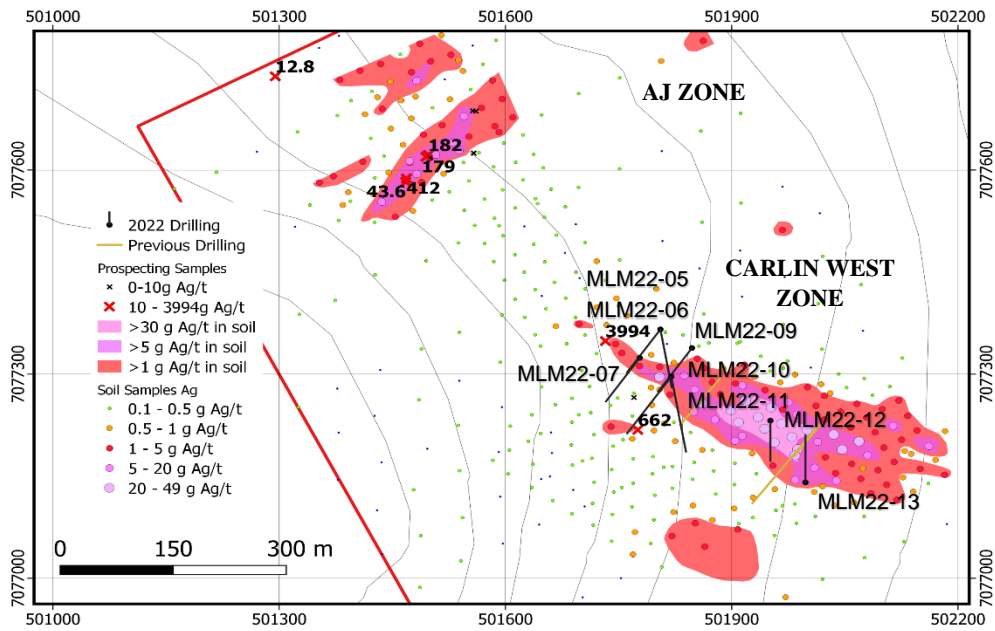
Carlin-Roop Project. Location of DDHs awaiting assays, AJ and Carlin West zones and recently enlarged 125m by 155m ( \geq 1\text{oz Ag/t} )
